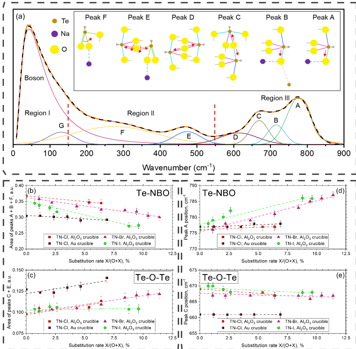
Figure 1. (a) Typical Raman spectrum of a sodium tellurite glass. The vibrational modes attributed to each peak are shown schematically. Dependence on the halogen contents and crucible materials of the area of peaks ascribed to (b) Te-NBO vibrational modes (peaks A, B, and F), and (c) Te-O-Te vibrational modes (peaks C and E). Dependence on the halogen contents and crucible materials of the peak position of (d) Te-NBO vibrational modes (peak A), and (e) Te-O-Te vibrational modes (peak C).
