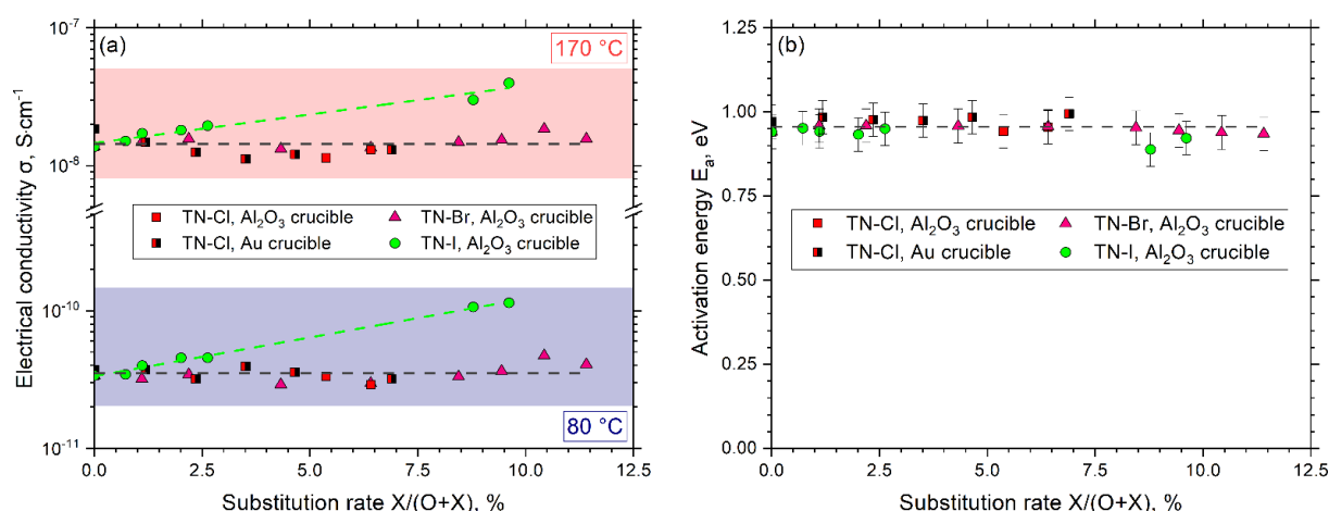
Figure 2. (a) Electrical conductivity at 80 and 170 °C, and (b) activation energy for electrical conductivity of TN-X-SR glasses with increasing halogen contents and varying crucible materials.
