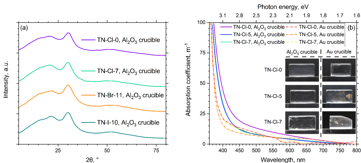
Figure 1. (a) XRD patterns of TN-X-SR glasses synthesized in \text{Al}_2\text{O}_3 crucibles. (b) UV-Vis absorbance spectra of TN-Cl-SR glasses with increasing halogen contents and varying crucible materials. The inset presents photographs of 2 to 3 cm wide specimens.
